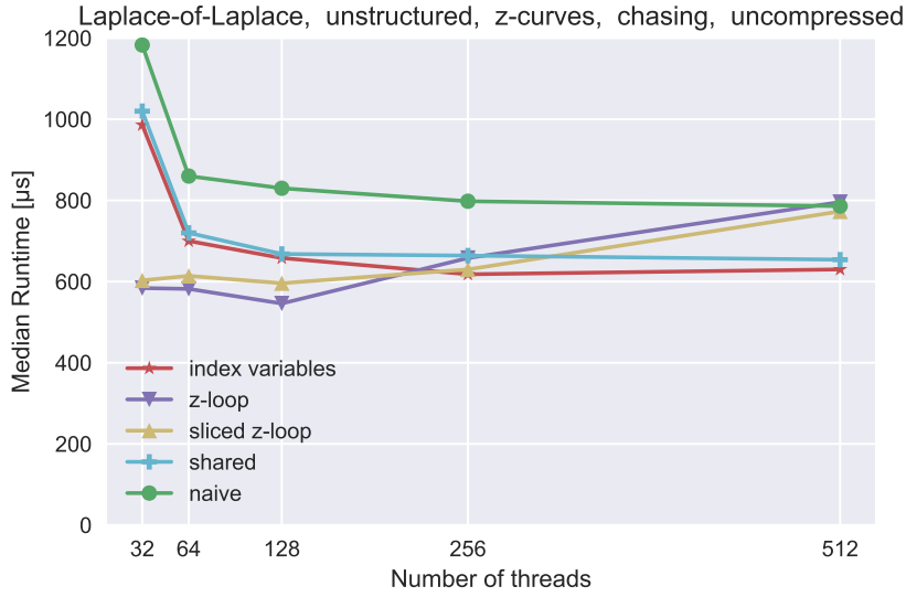
Figure 6.4: Impact of the total number of threads on the runtime for different implementations of the laplap stencil ( 512 \times 512 \times 64 grid, z-curves memory layout with double precision, chasing and uncompressed neighborhood table).
