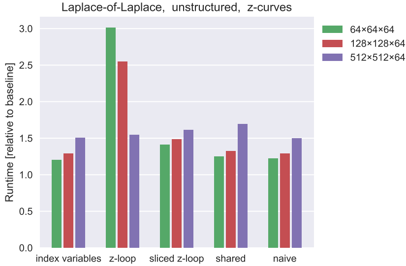
Figure 6.6: Relative overhead compared to the fastest regular variant of different implementations of the laplap stencil on an unstructured grid with z-curves memory layout. For each bar, the fastest neighborhood table implementation was plotted (i.e. all combinations of compressed and uncompressed , chasing and non-chasing were benchmarked and the fastest setup was chosen). Baseline: fastest regular grid implementation.
